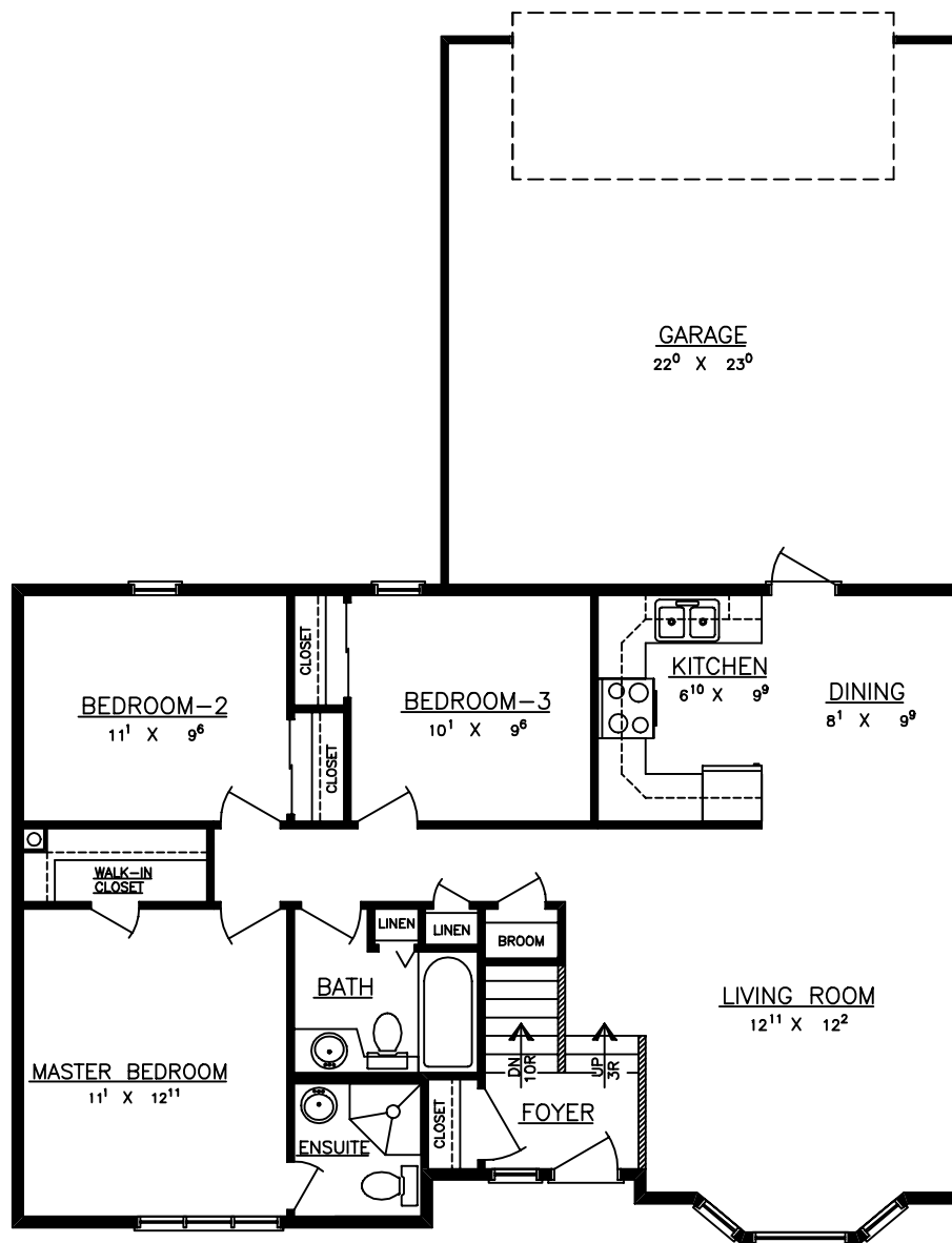
FLOOR PLAN
